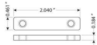
Track Nut
